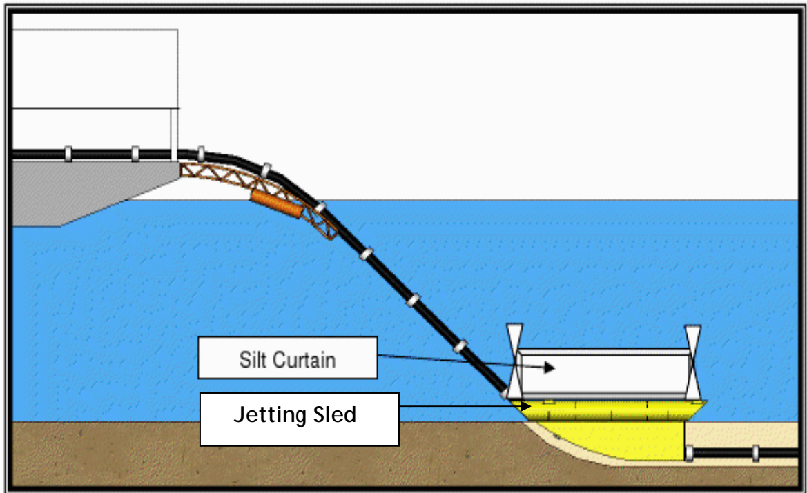
FIGURE 4.5 : SUBMARINE PIPE INSTALLATION WITH JETTING SLED
